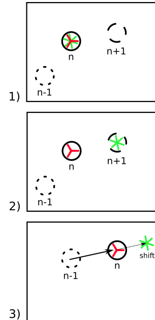
Figure 2: The three phases of the SceneWalk model. The circles indicate fixation positions, with n being the current. The green, 5-pointed star is the center of the attention Gaussian while the red, 3-pointed star is the center of the inhibitory Gaussian. Panel 1 shows the main fixation phase, where fixation position and the Gaussians align. In Panel 2 the center of the attention Gaussian moves to the upcoming fixation position, modelling a presaccadic attention shift. Panel 3 shows the post-saccadic attention shift where attention shifts in the direction of the saccade after fixation onset. After the post-saccadic phase, attention moves to the current fixation position, establishing the same situation as in Panel 1.
