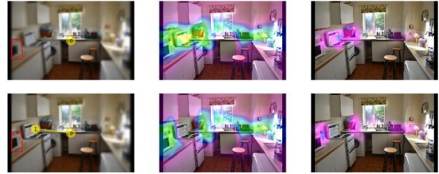
Figure 6: IRL model searching for a microwave target (red box) in a test image. Right, action maps. Middle, reward maps. Left, cumulative ReT-images based on the first fixation (top row) and second fixation (bottom row).
