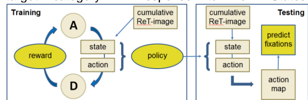
Figure 1: The adversarial IRL model of categorical search.
