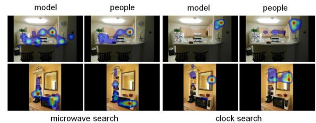
Figure 7: Fixation-density maps from the model and people searching for a microwave (left 4 panels) and clock (right 4).
